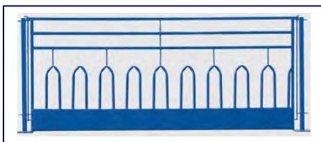
TFG FEED FRONT for goats 8" skirt keeps muck out of feed 40" high 24" to top of tombstone Post sold separately on feeder fronts
