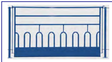
TFS FEED FRONT for sheep Designed for floor feeding 8" skirt keeps muck out of feed 40" high 20" to top of tombstone
